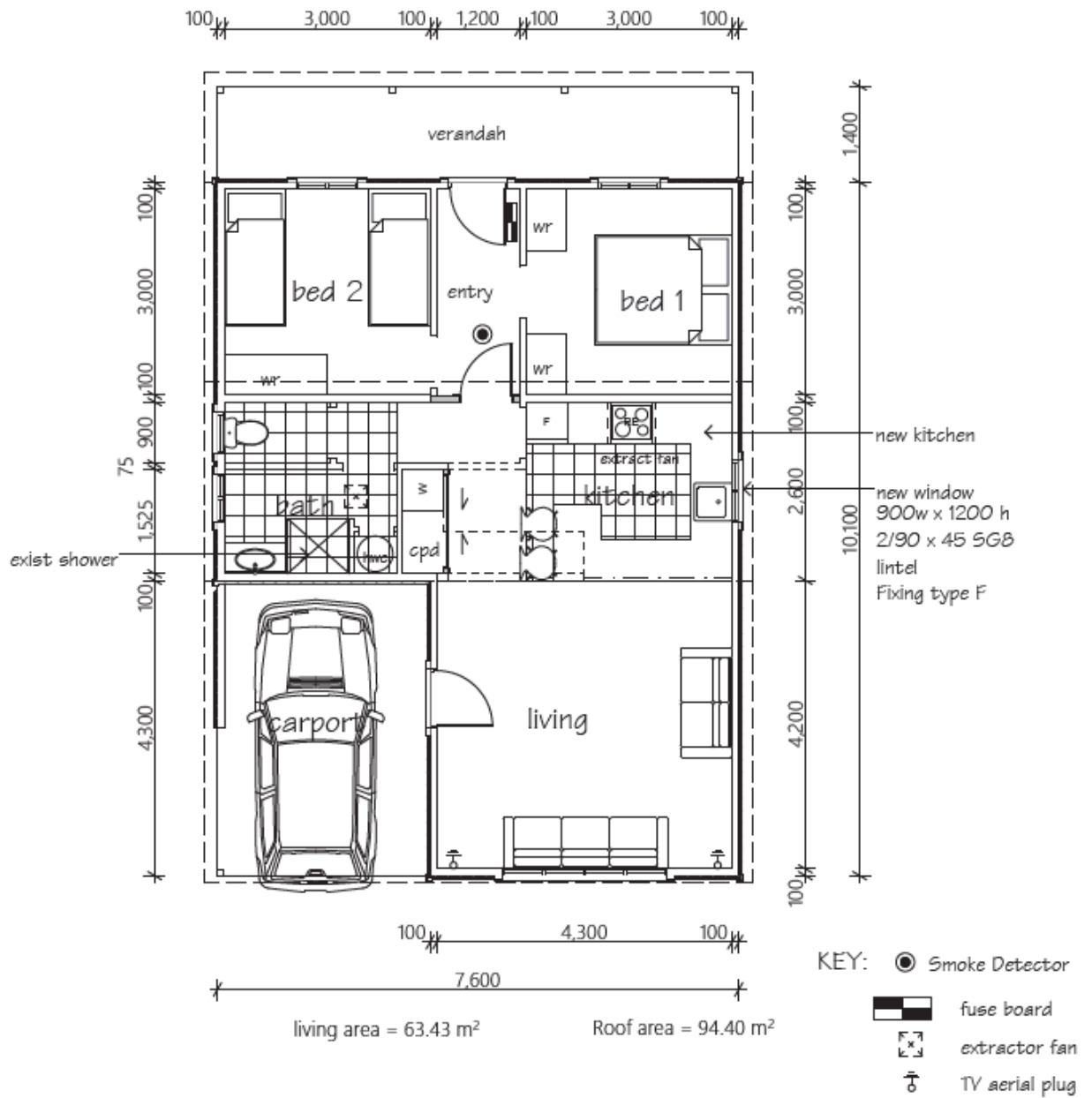
1. Proposed Floor 1:100
