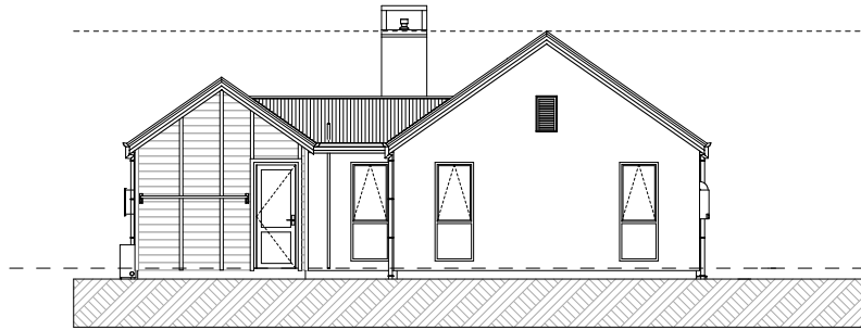
South Elevation
