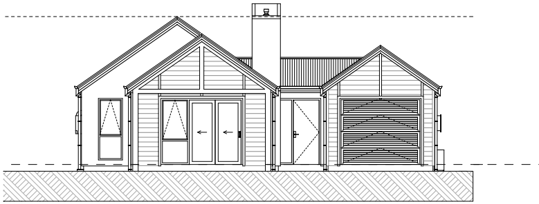
North Elevation
