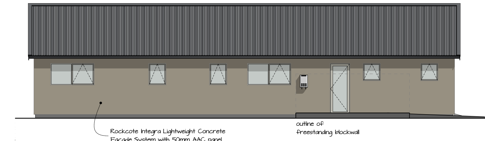
E-02 East Elevation 1:100
