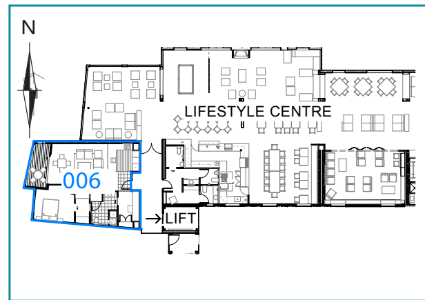
Ground Floor Plan - Stage Three
